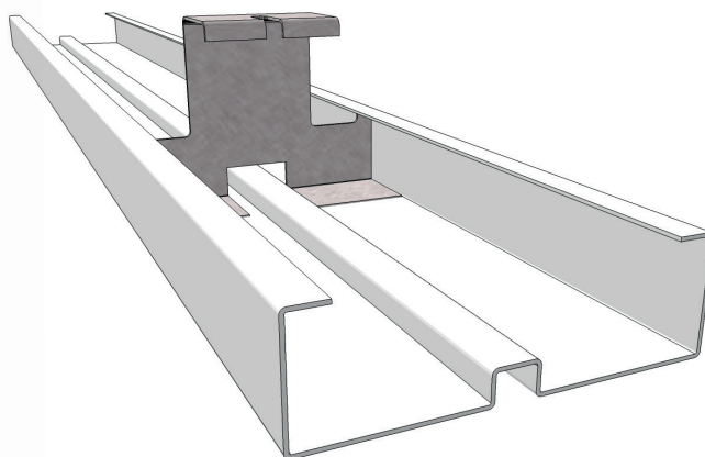
Rail C joint creux
